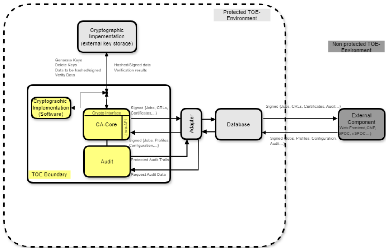
Figure 1: TOE boundary
