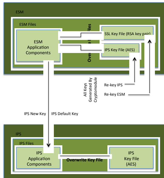
Figure 4: IPS and ESM Keying
