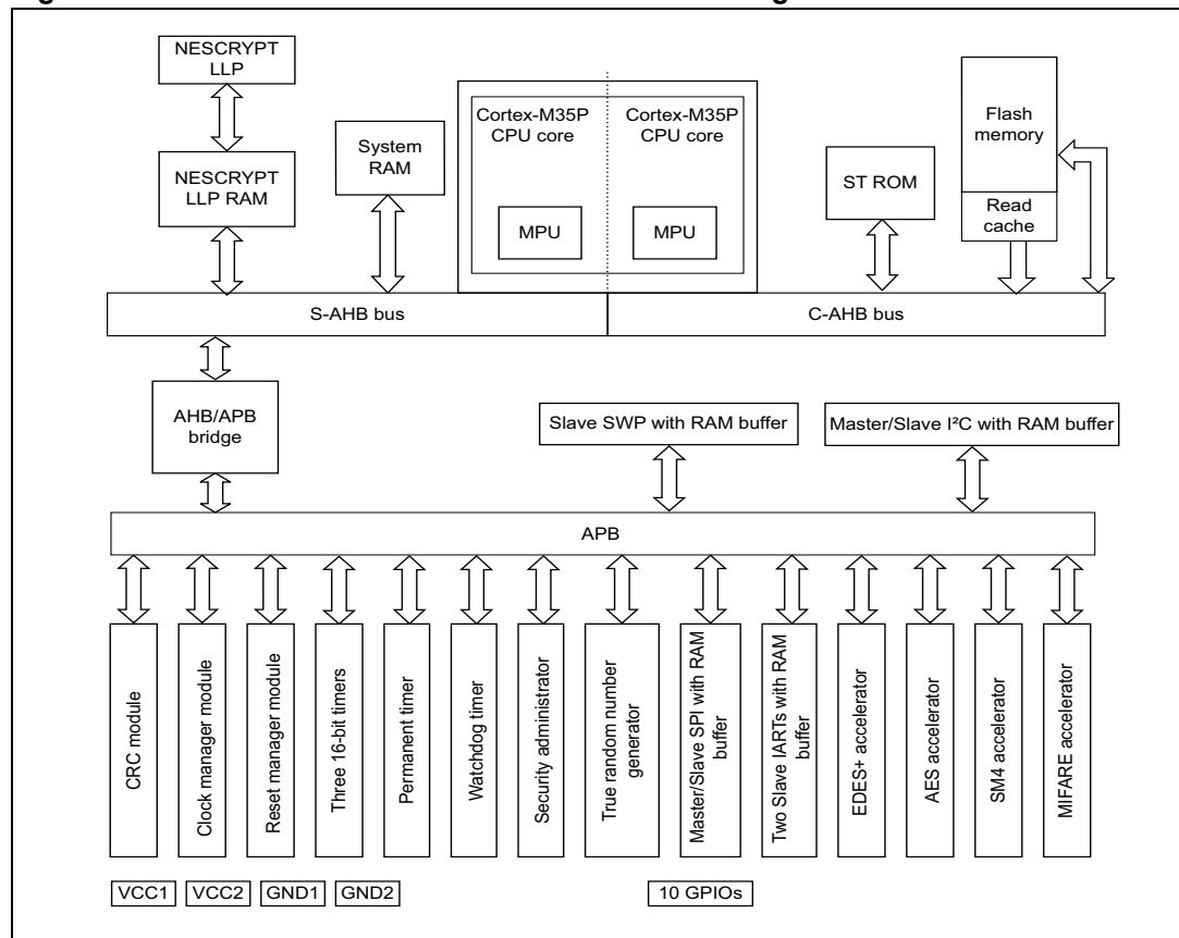
Figure 1. ST33K1M5C and ST33K1M5T A02 block diagram
