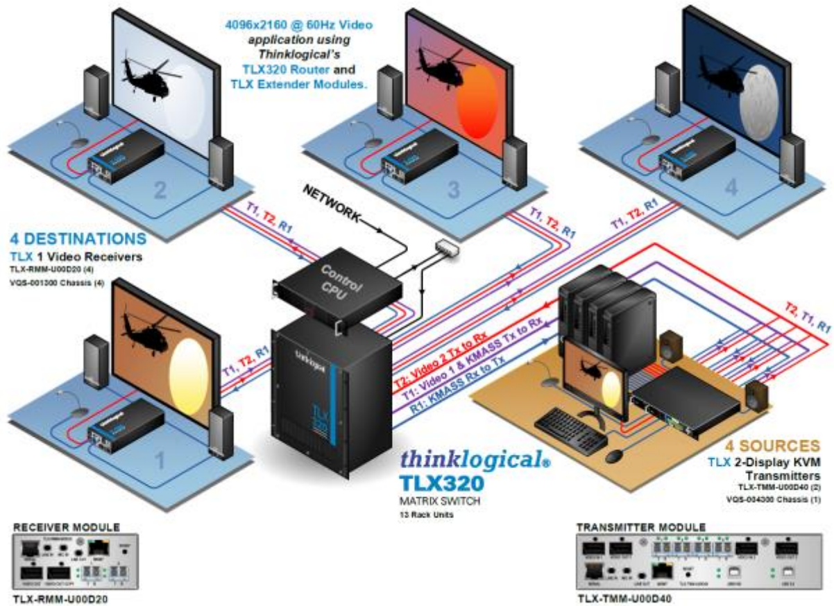
2a. Typical TOE TLX320 Configuration
