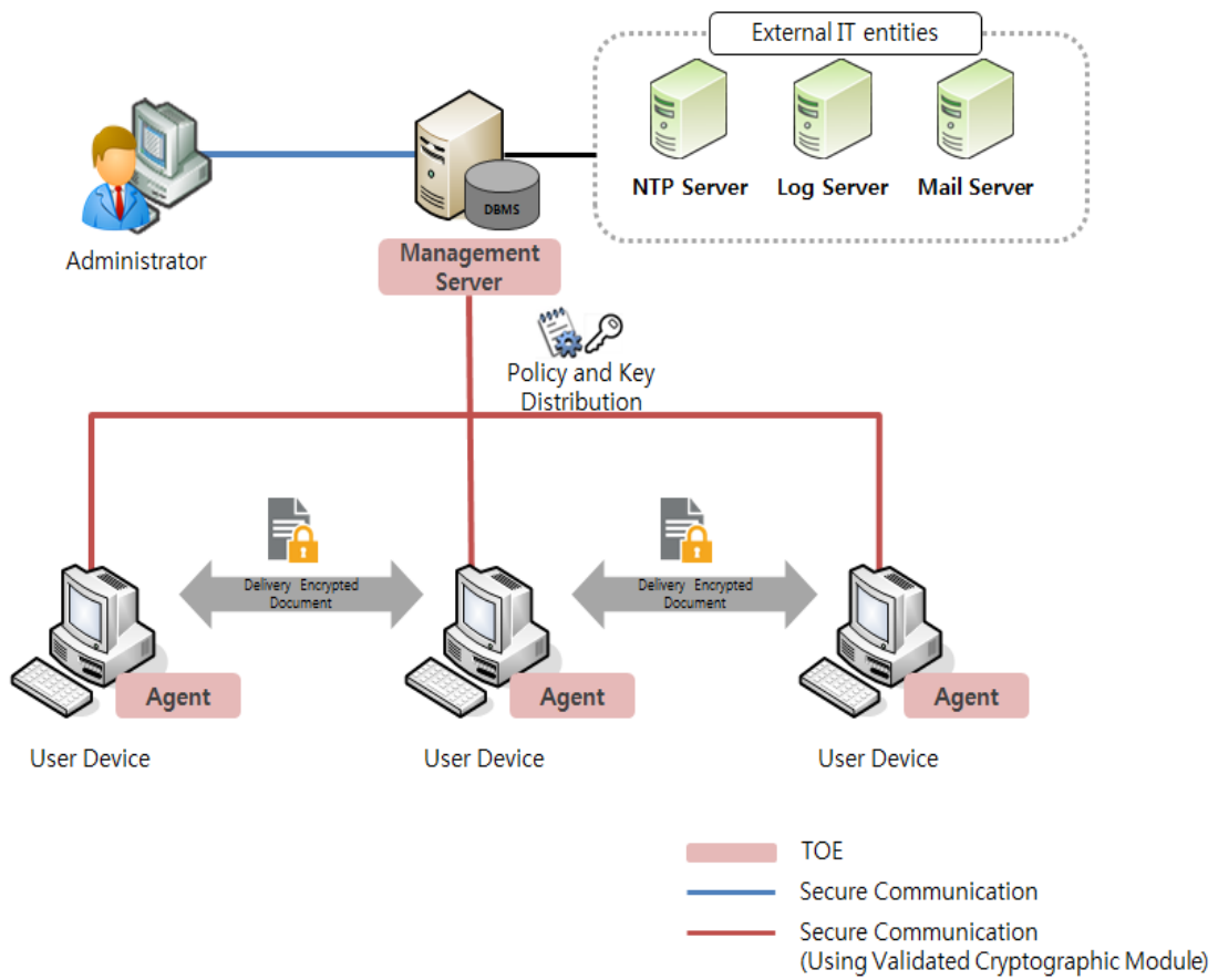
[Figure 1] Operational environment of Electronic Document Encryption (1)
