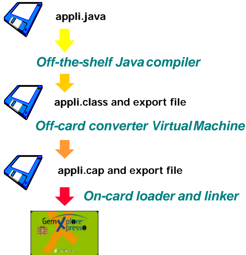
Figure 3 – Applet verification
