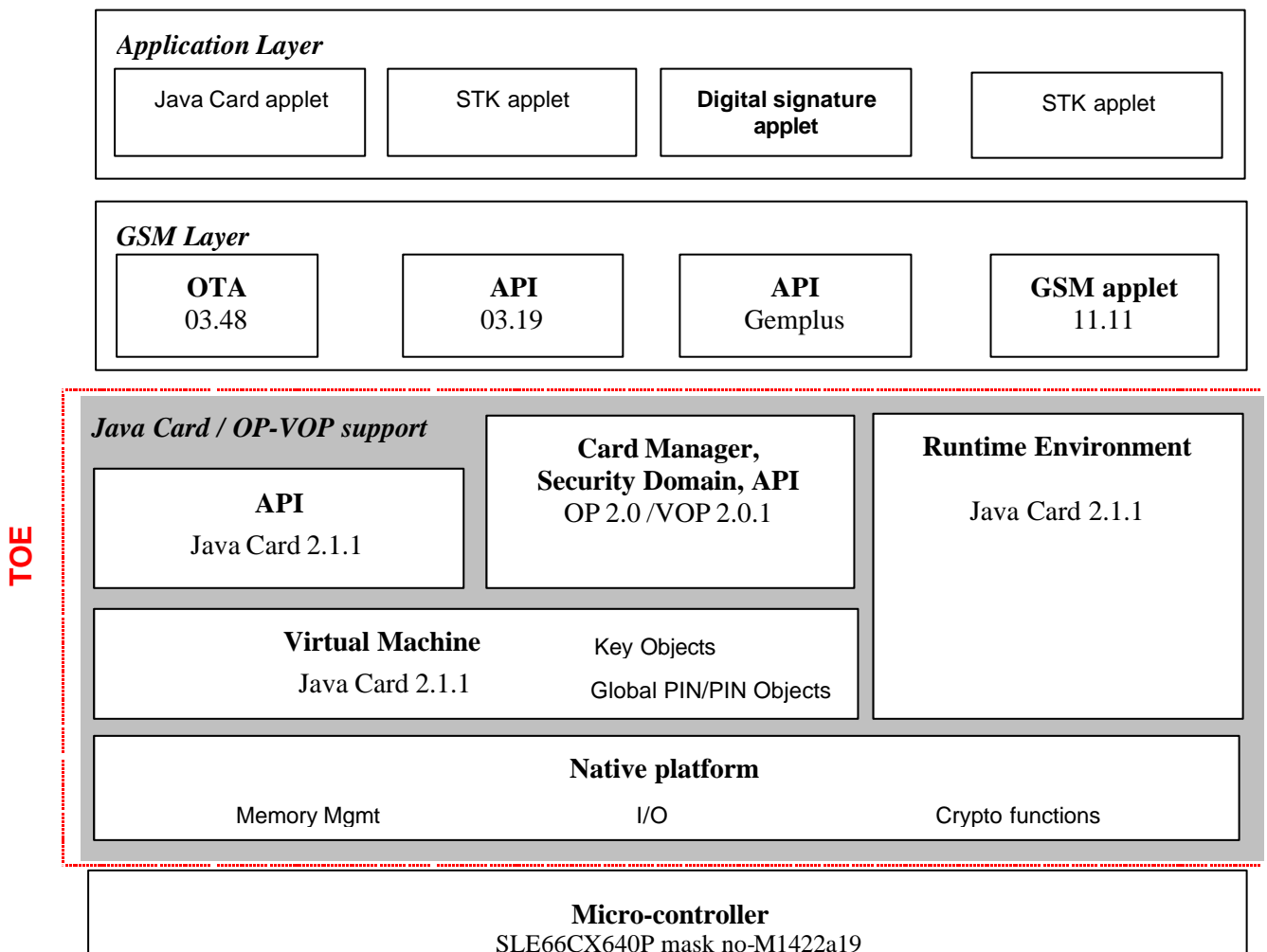
Figure 1 – TOE Architecture
