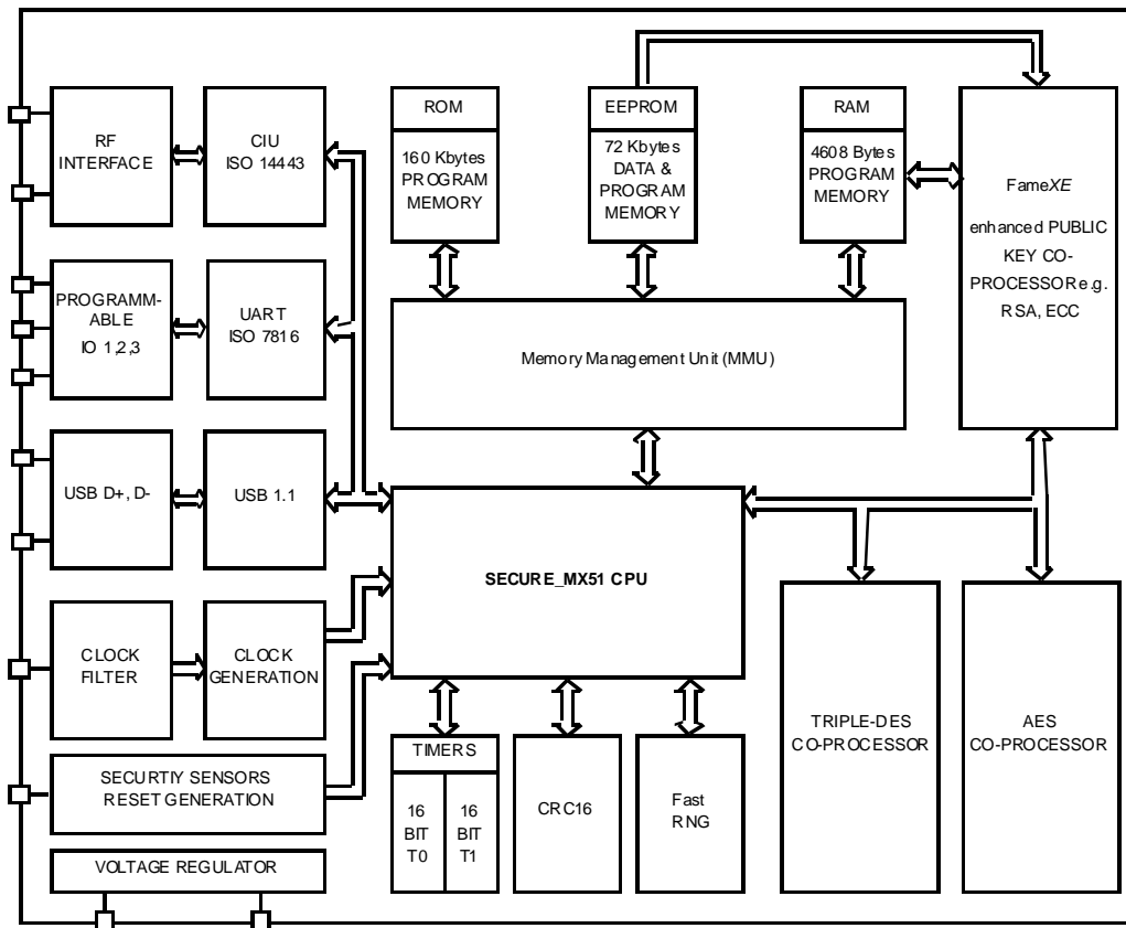
Figure 1: Block Diagram of the P5CT072V0M
