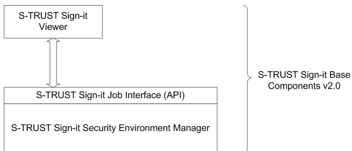
Figure 1 Architectural Overview
