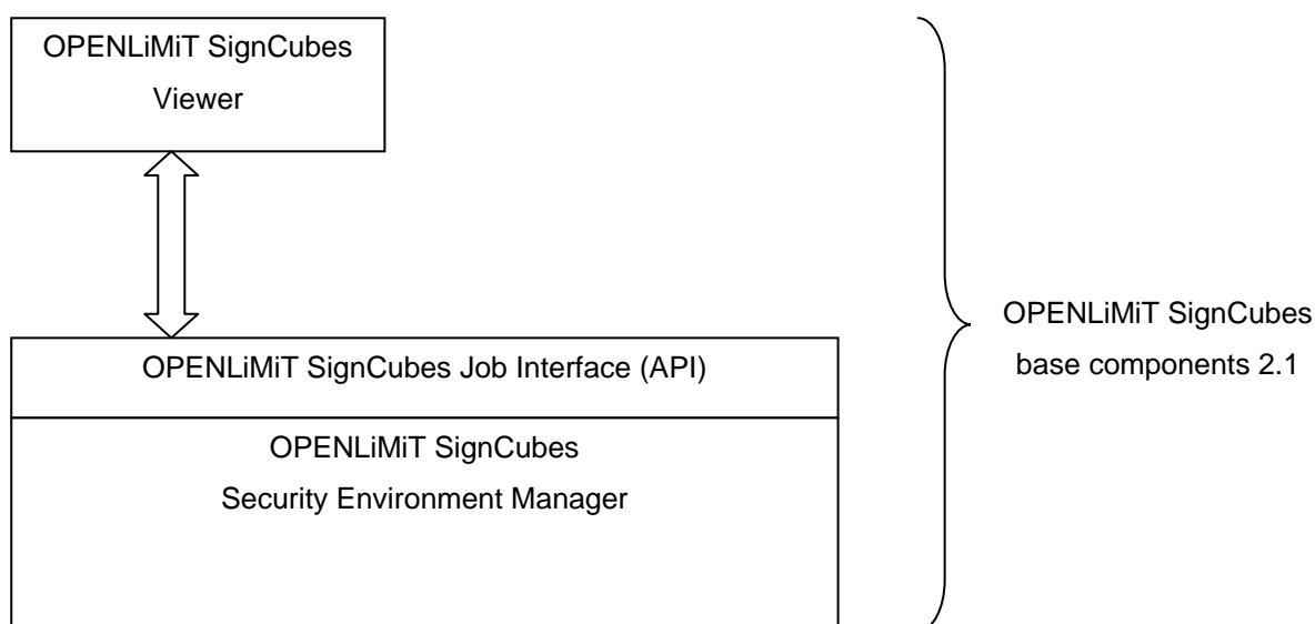
Figure 1 Architectural Overview
