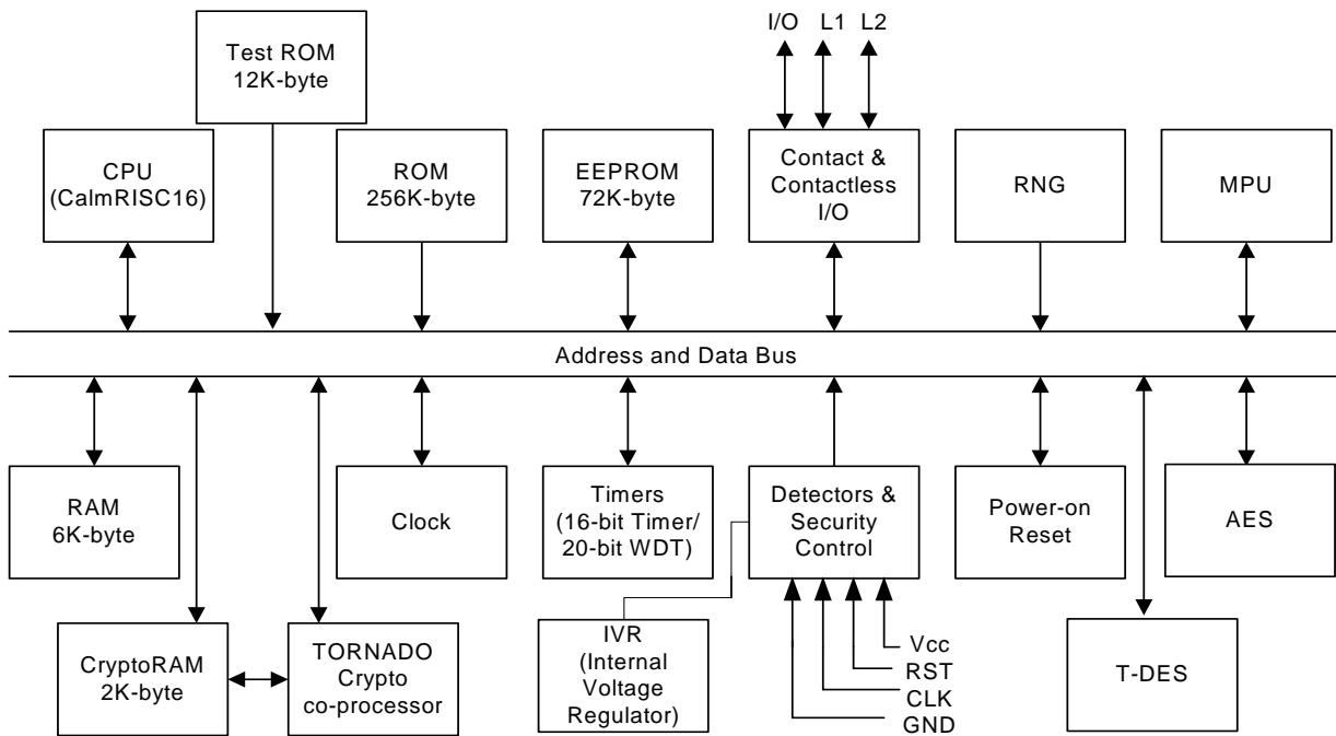
Figure1. S3CC9GC Block Diagram
