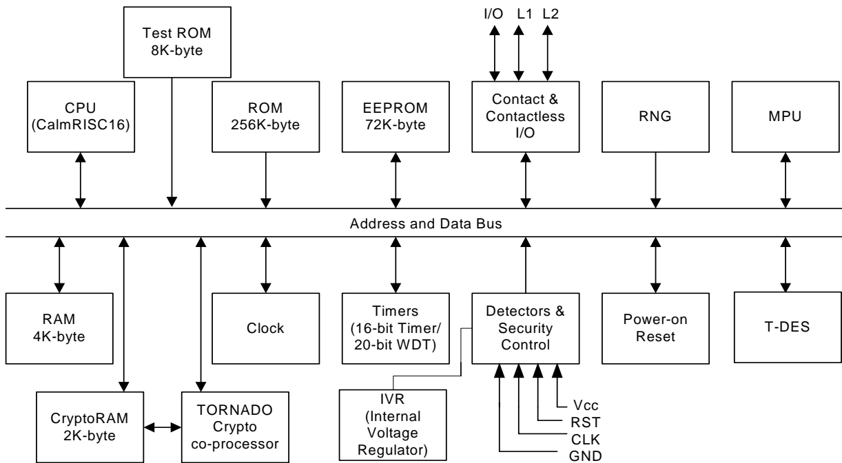
Figure1. S3CC9LC Block Diagram
