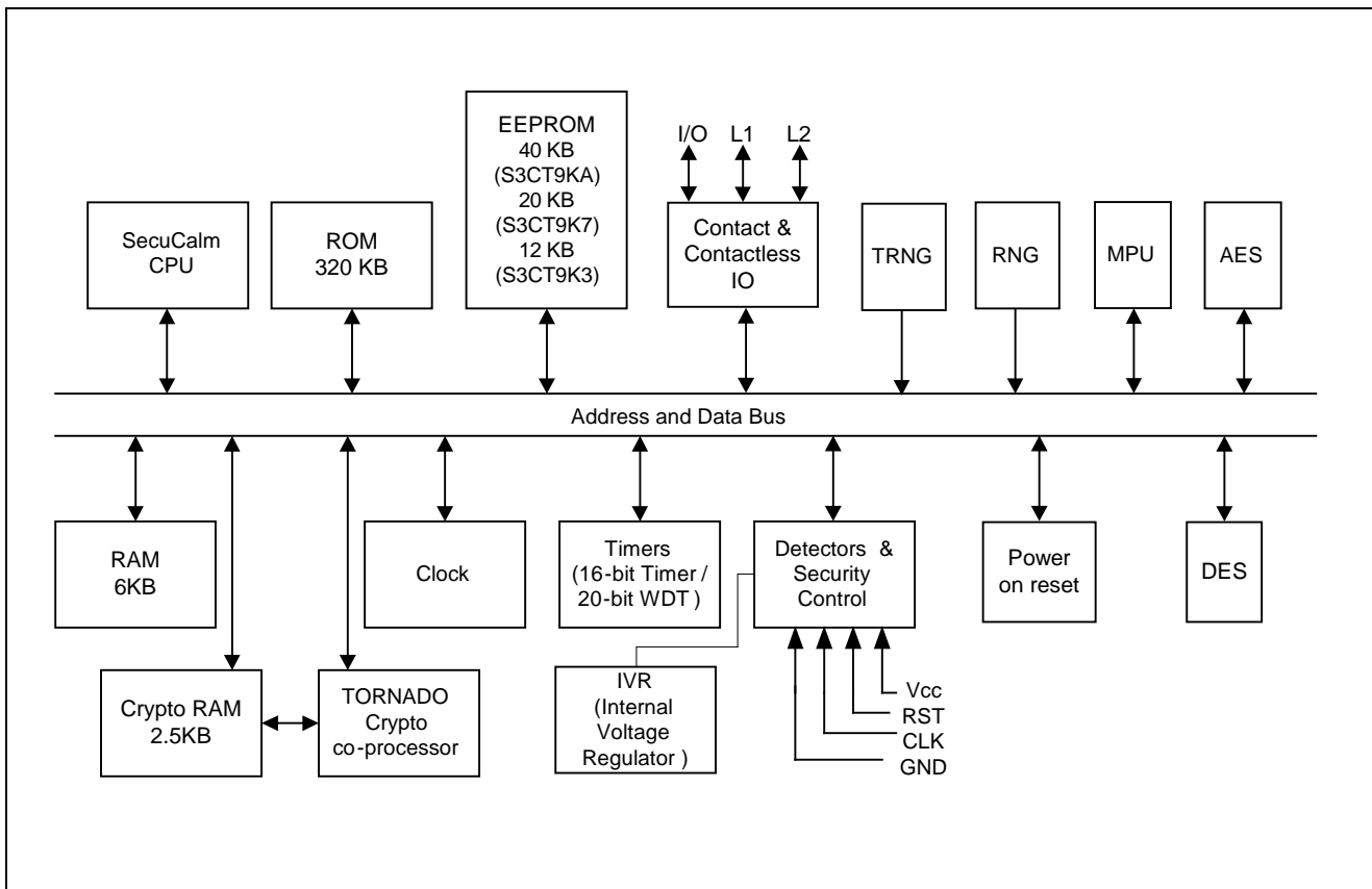
Figure 1. S3CT9KA/ S3CT9K7/ S3CT9K3 Block Diagram
