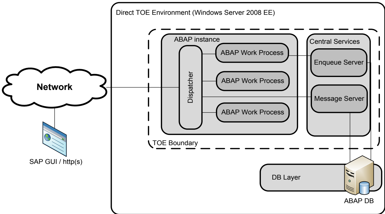
Figure 2: System Architecture of a minimal installation
