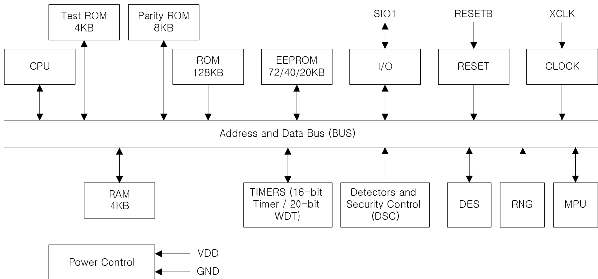
Figure 1 S3CT9AC/S3CT9AA/S3CT9A7 Block Diagram
