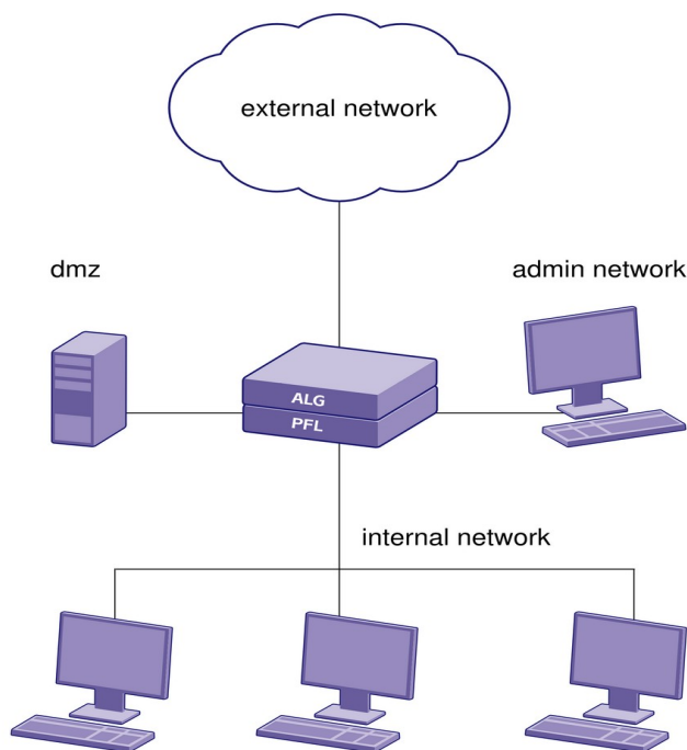
Figure 1.1: genugate 9.0 Z overview. The secure server network is labelled as dmz.
