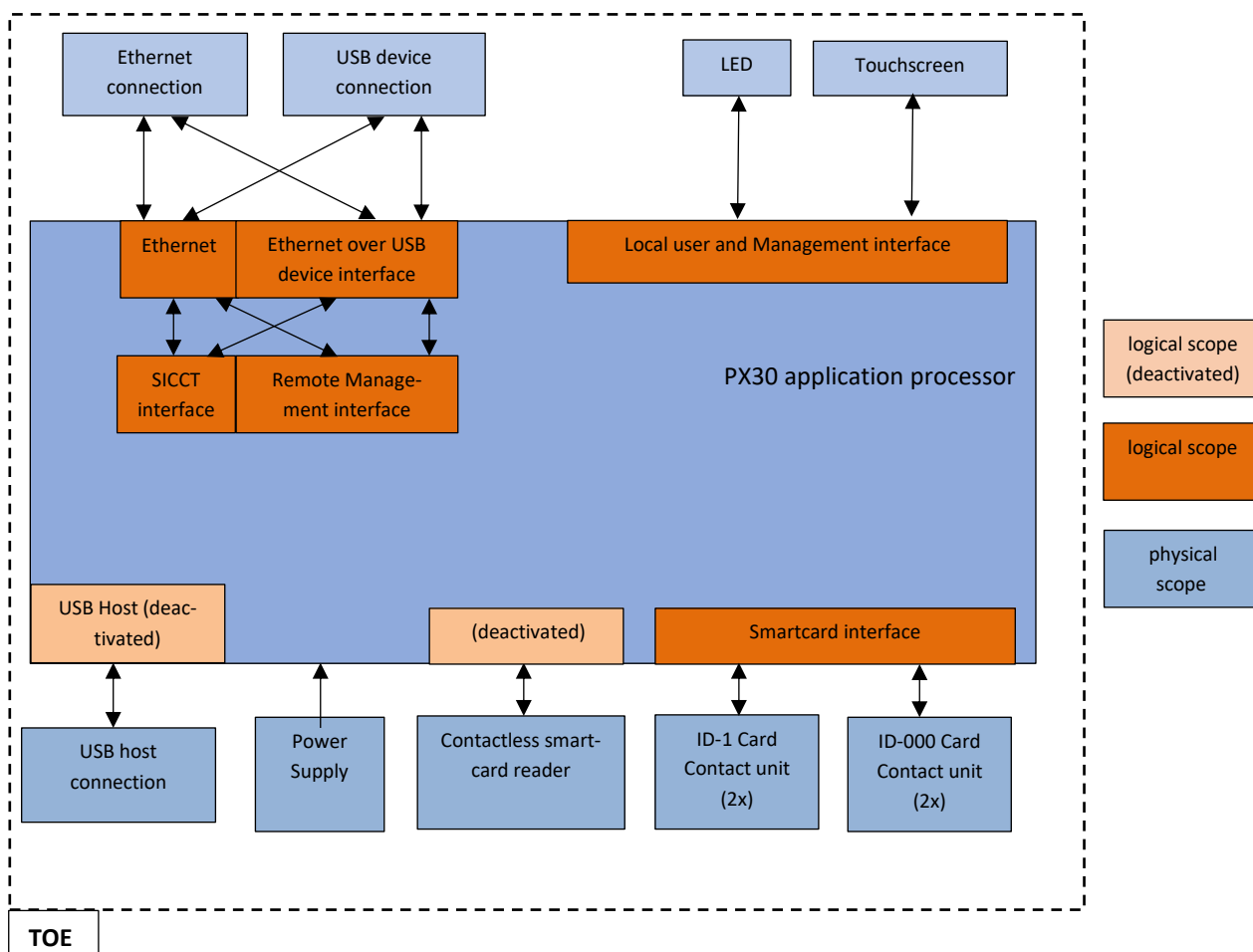
FIGURE 1.2: SCHEMATIC REPRESENTATION OF THE TOE, SHOWING ALL EXTERNAL
