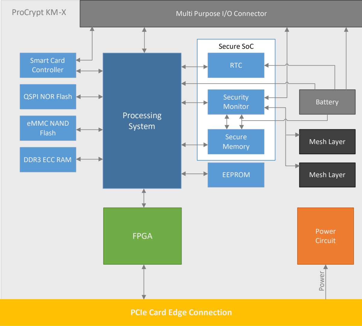
Figure 2: TOE Hardware Architecture
