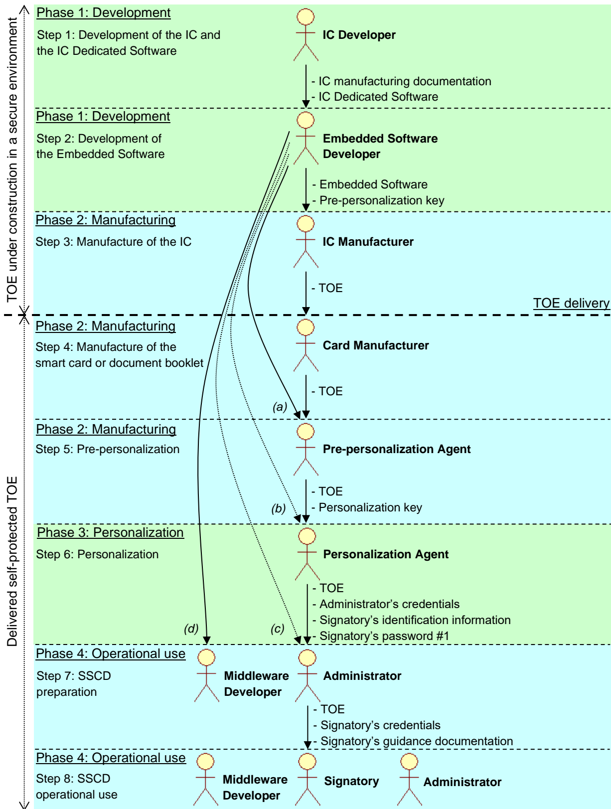
Figure 2-2 Life cycle of the TOE SSCD application
