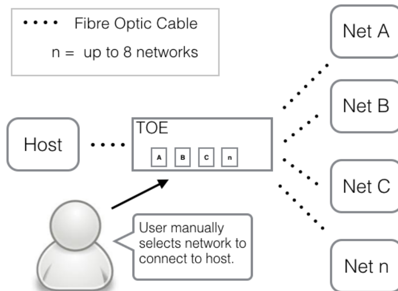
Figure 1 TOE Architecture
