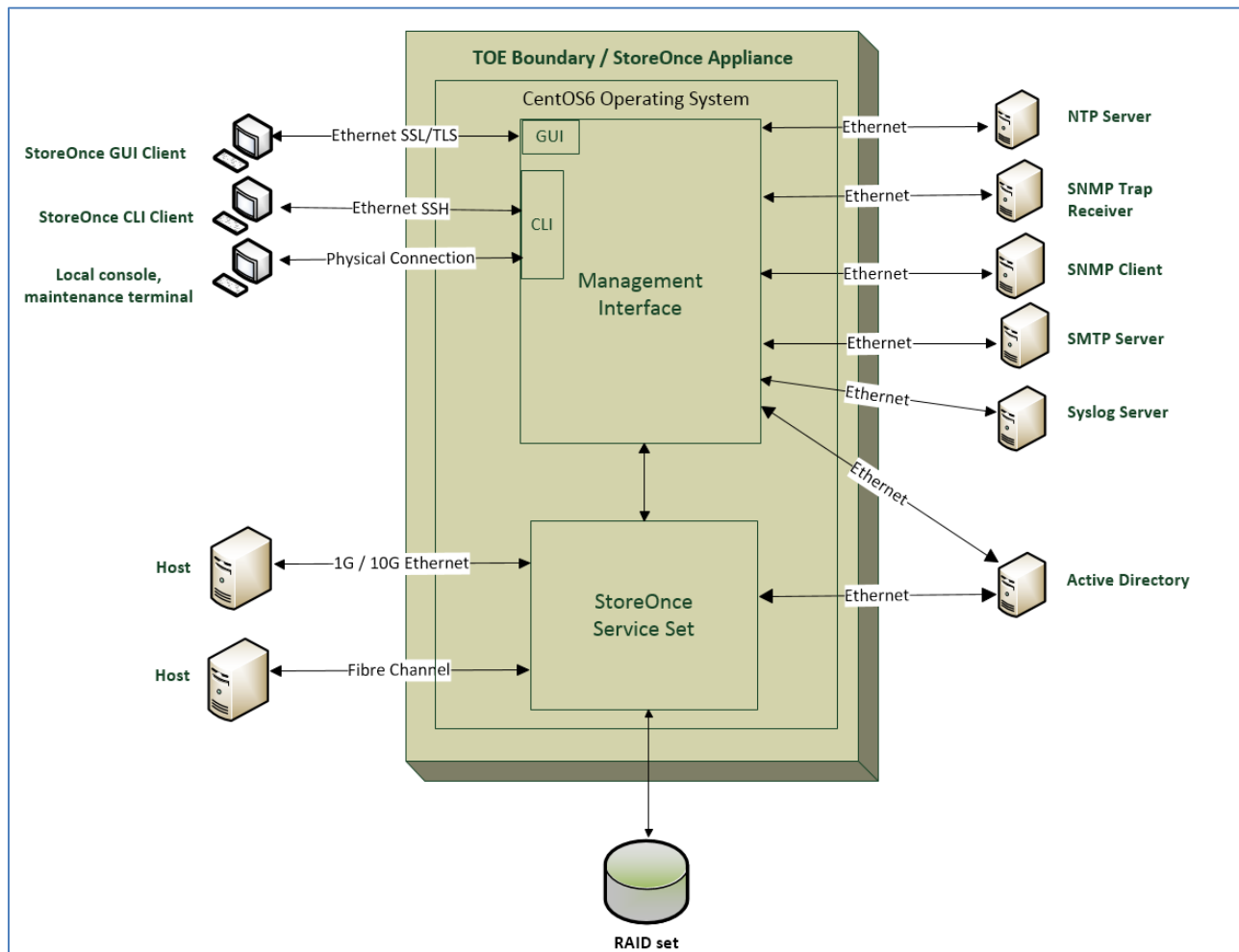
Figure 1 - HPE StoreOnce TOE Boundary
