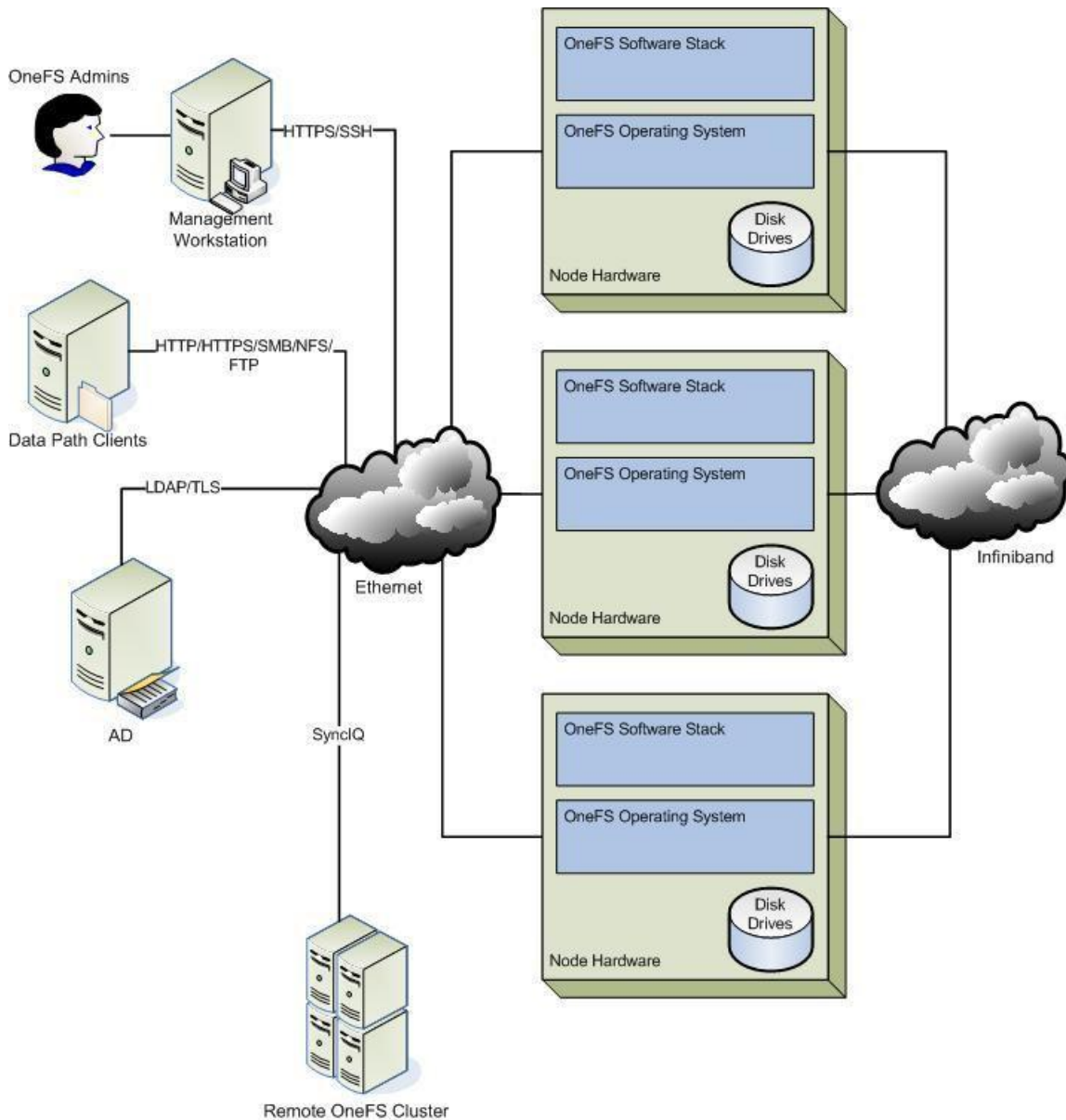
Figure 1 Deployment Configuration of the TOE
