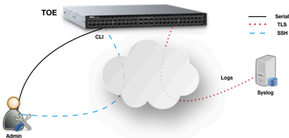
Figure 1: TOE Architecture
