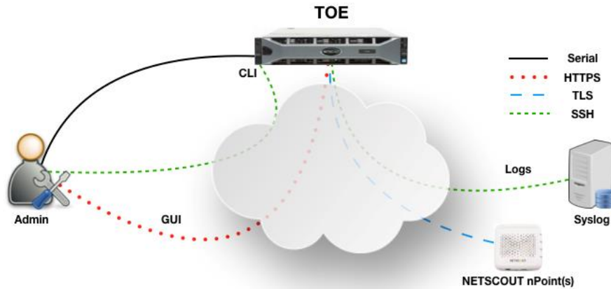
Figure 2: TOE interfaces
