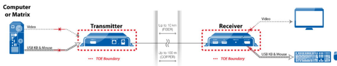
Figure 1: TOE Architecture
