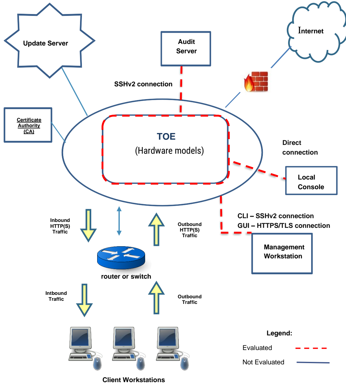
Figure 1: TOE Architecture
