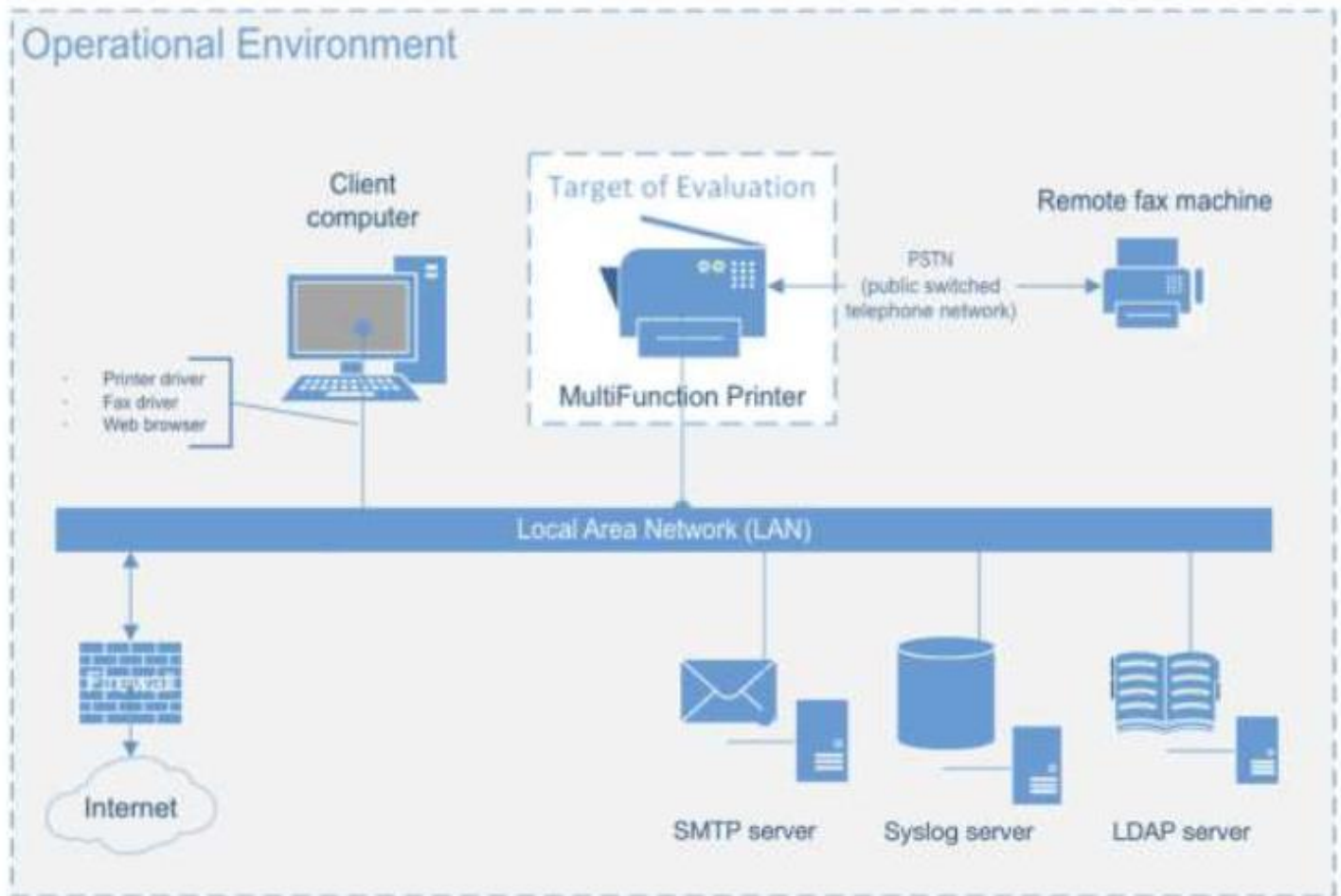
Figure 1: TOE Architecture
