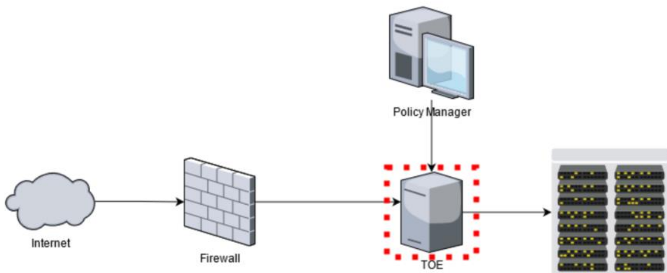
Figure 1: TOE Architecture
