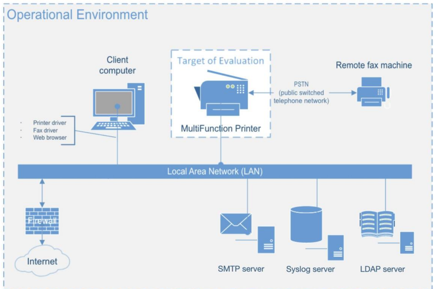
Figure 1: TOE Architecture
