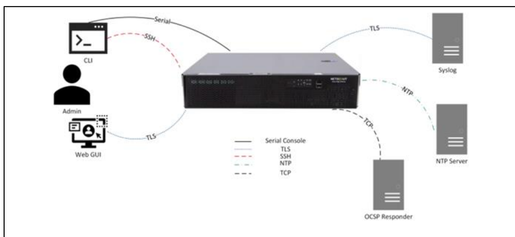
Figure 1: TOE Architecture
