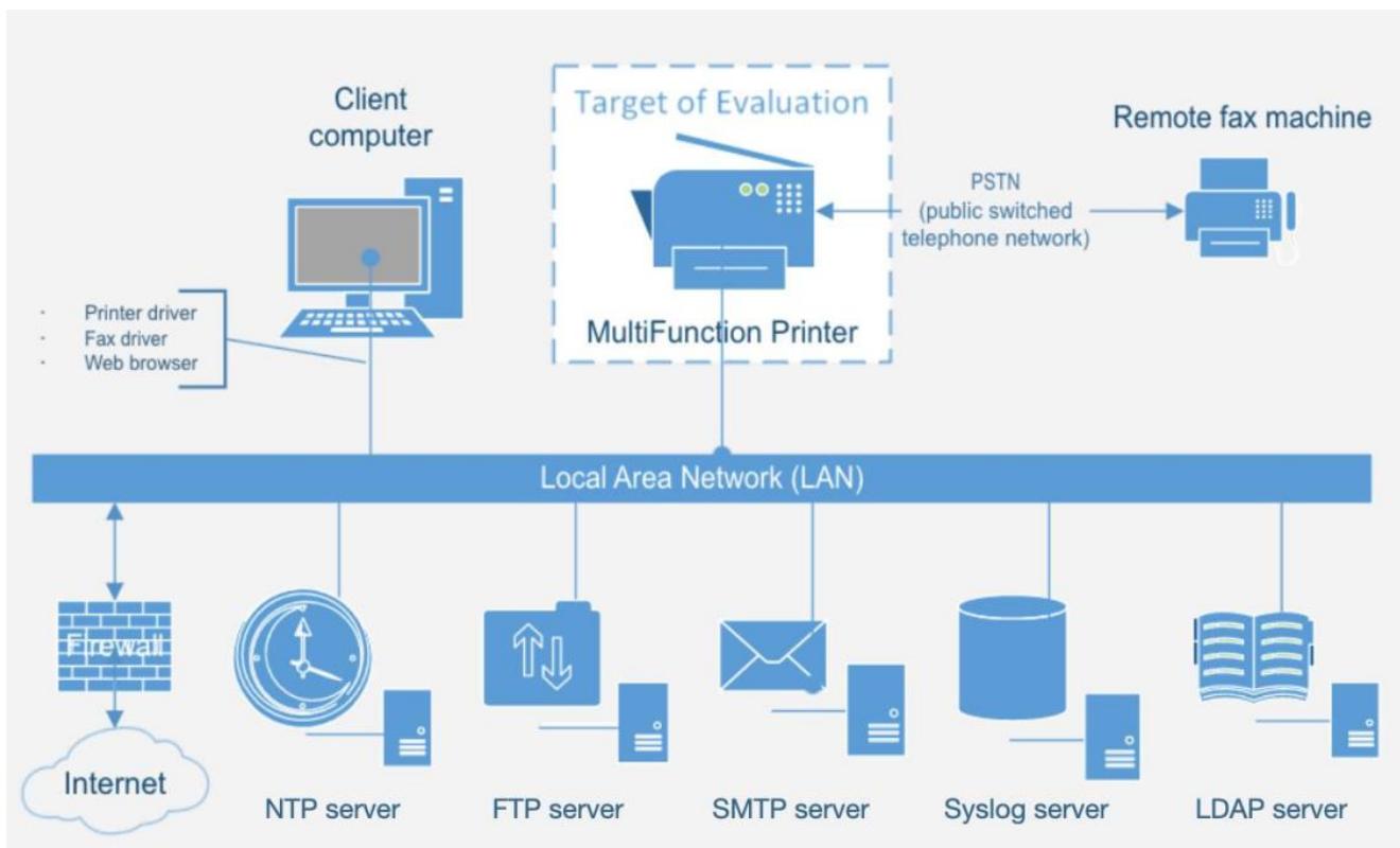
Figure 1: TOE Architecture
