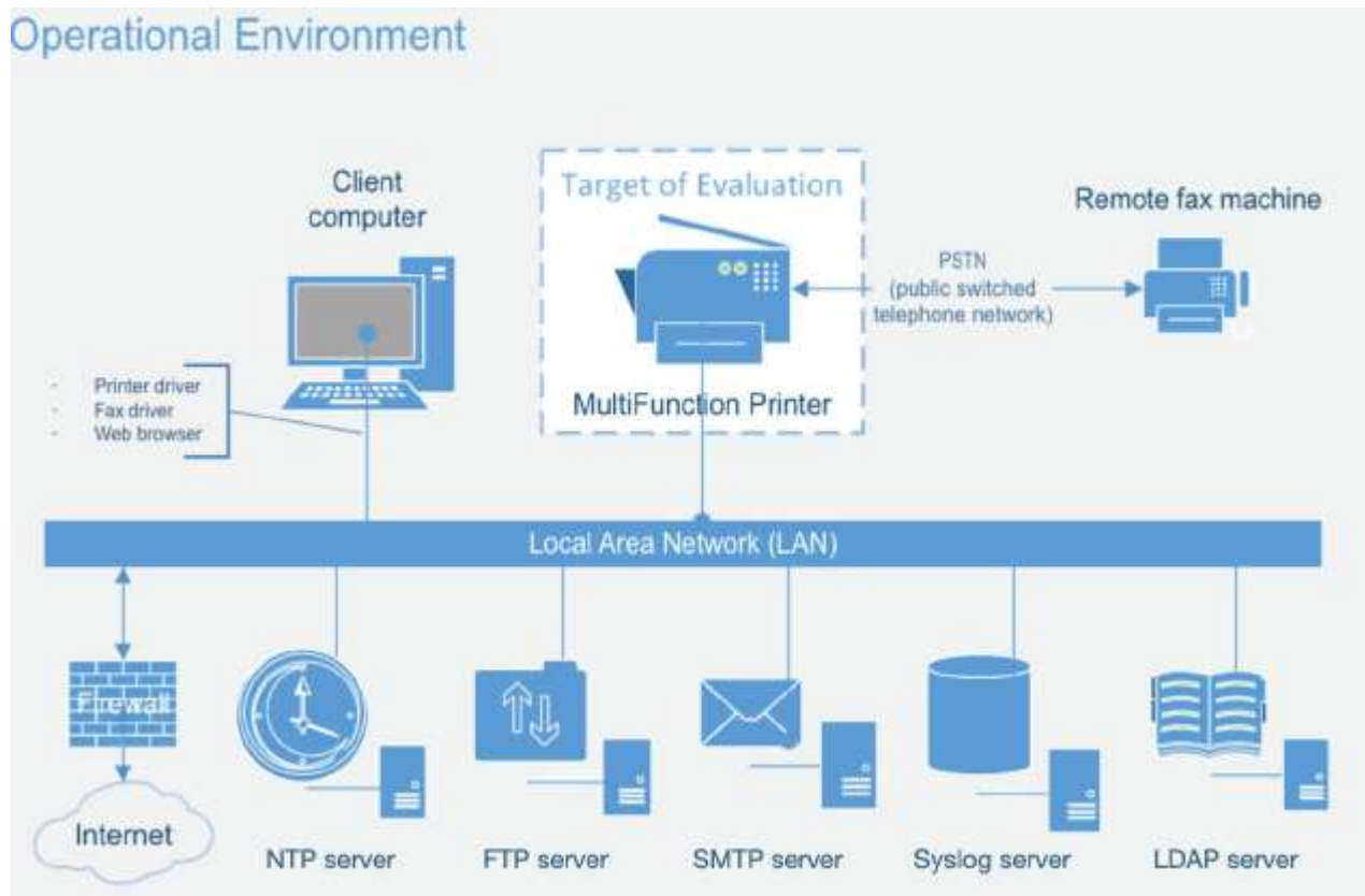
Figure 1: TOE Architecture
