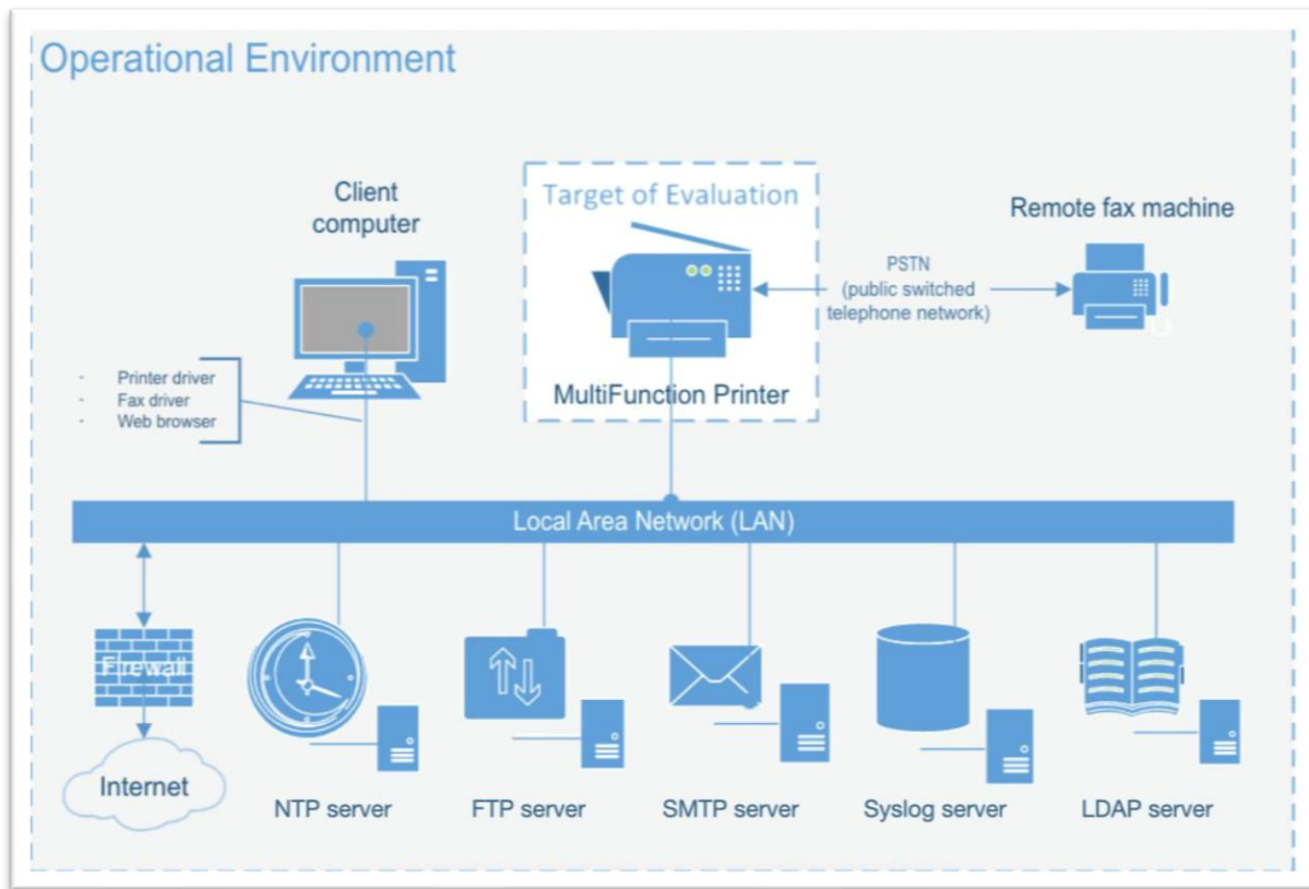
Figure 1: TOE Architecture
