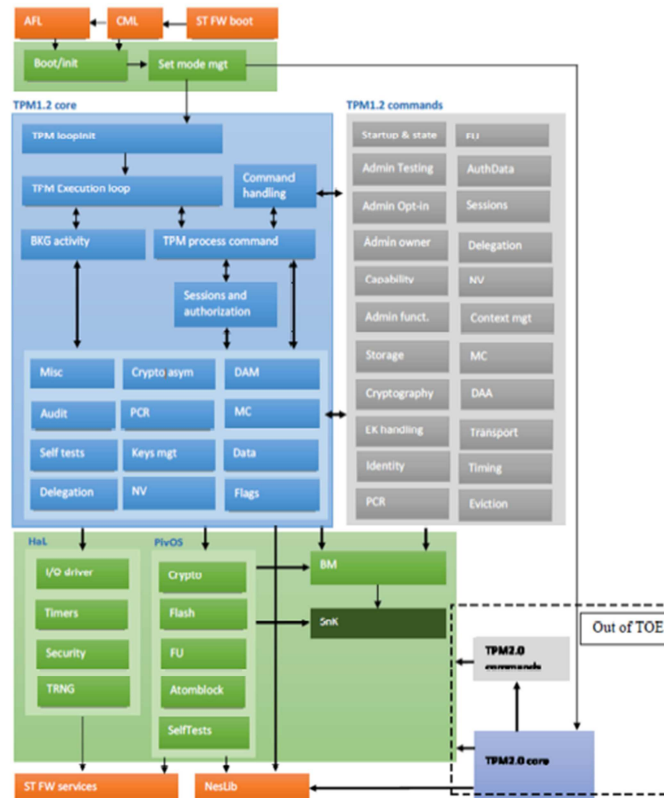
Figure 2 – Architecture firmware
