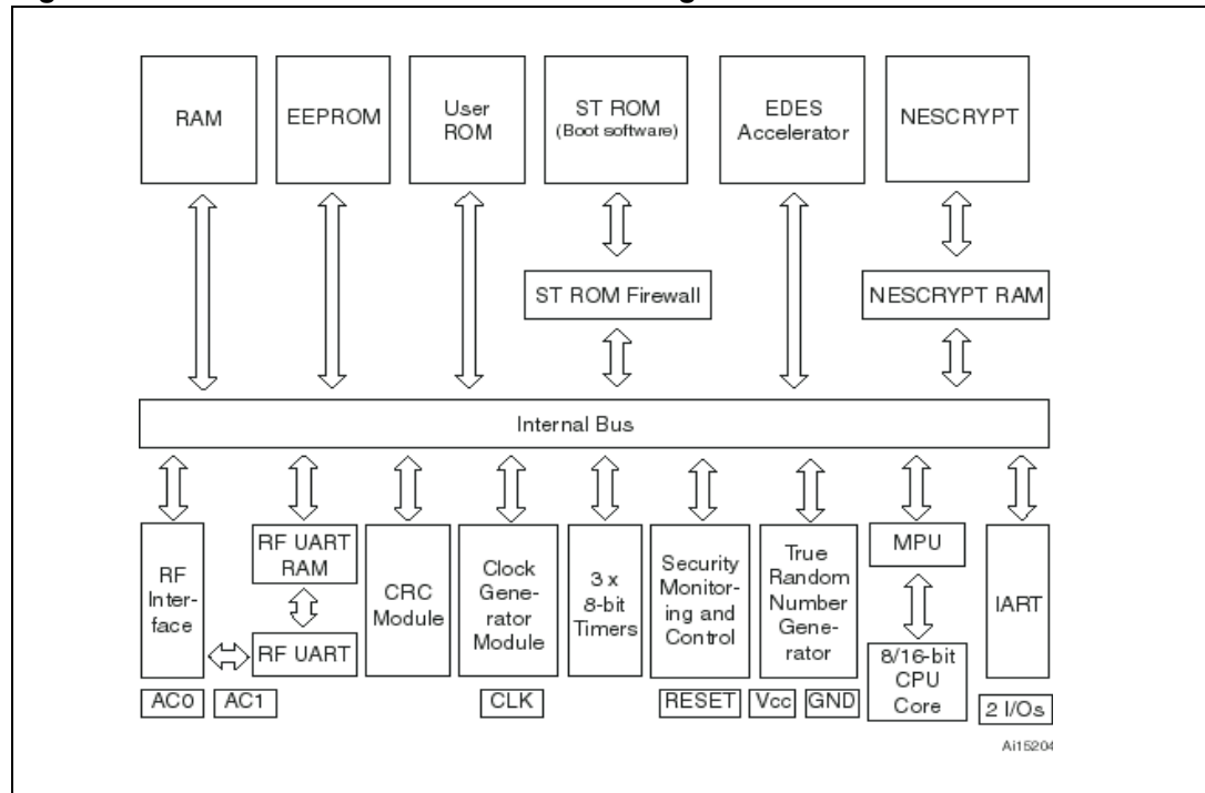
Figure 1. SA23YR18A / SB23YR18A block diagram
