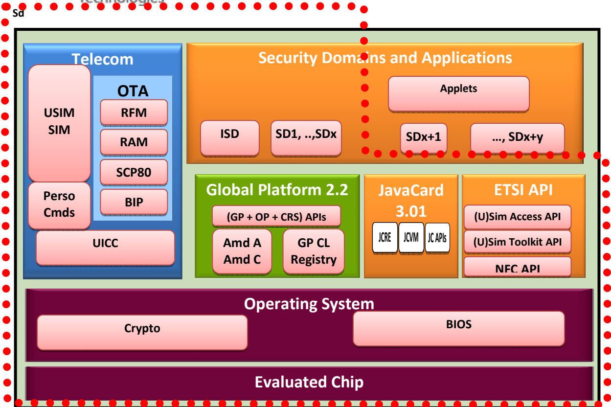
Figure 1: NFC FLYBUY Architecture
