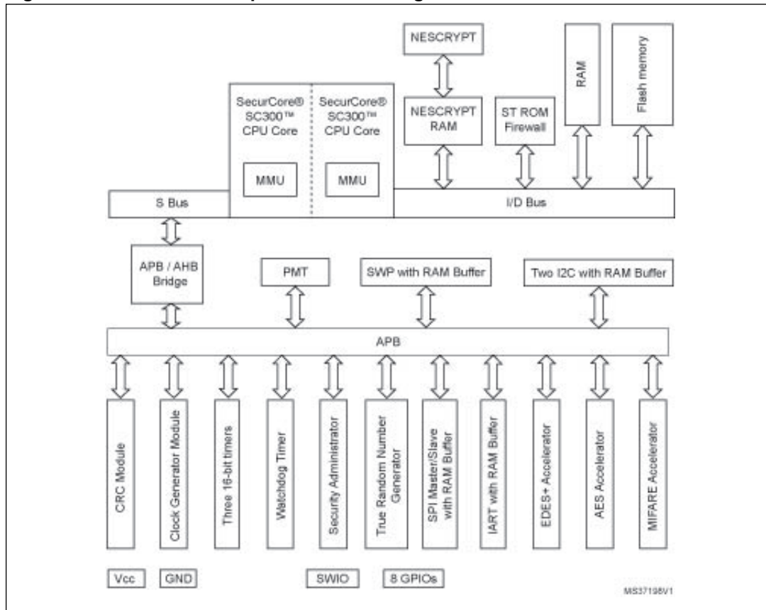
Figure 1. ST33J2M0 C03 platform block diagram
