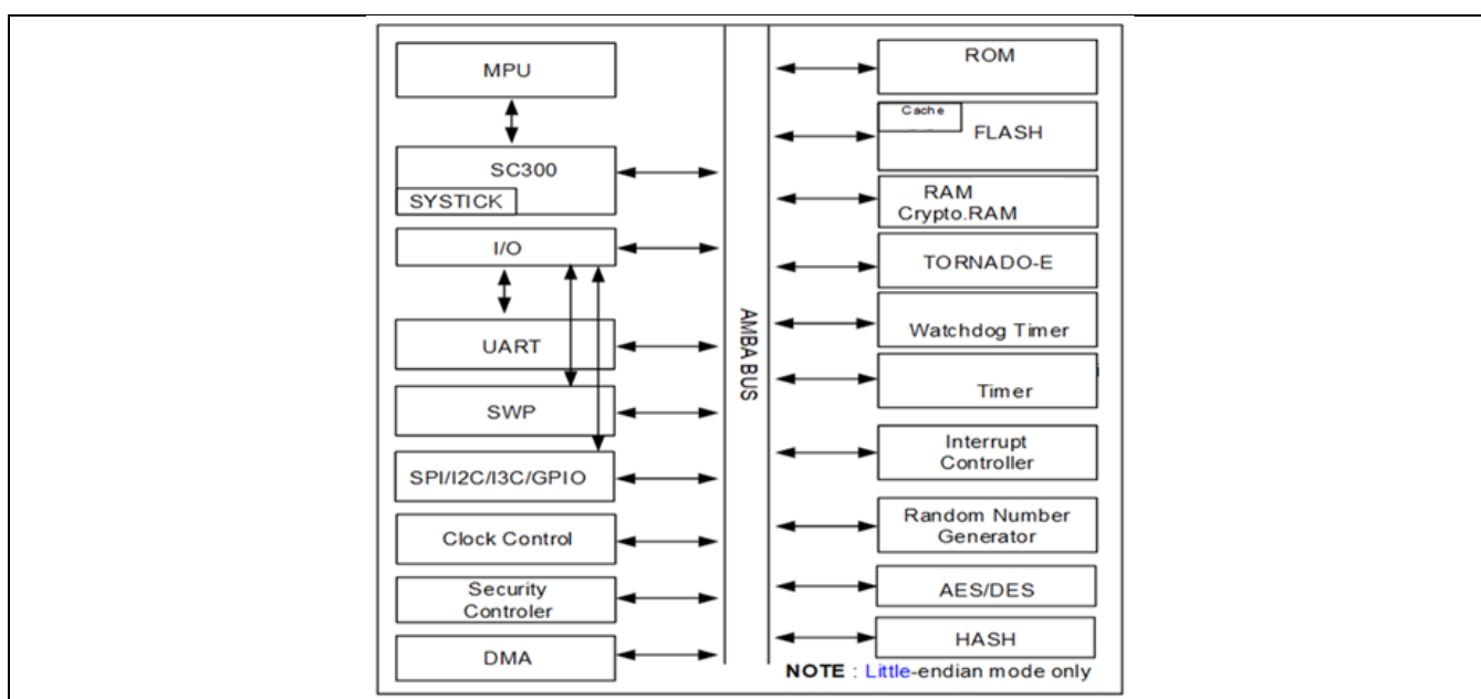
Figure 1 S3SSE1A Block Diagram
