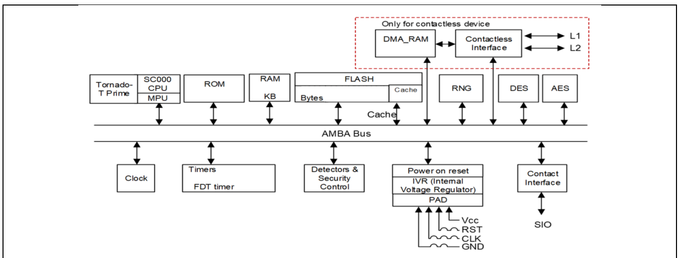
Figure 1 S3D384E/S3D352E/S3D300E/S3D264E/S3D232E/S3K384E Block Diagram
