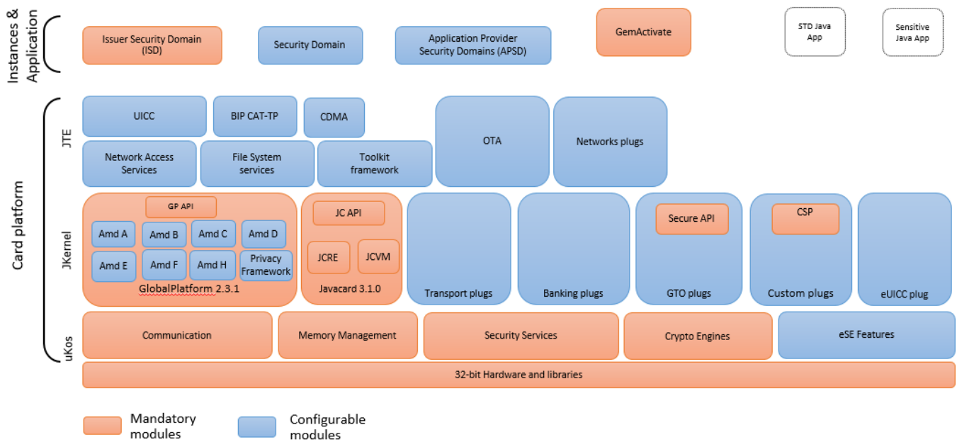
Figure 2: TESS v5.1 on S3NSEN6 architecture
