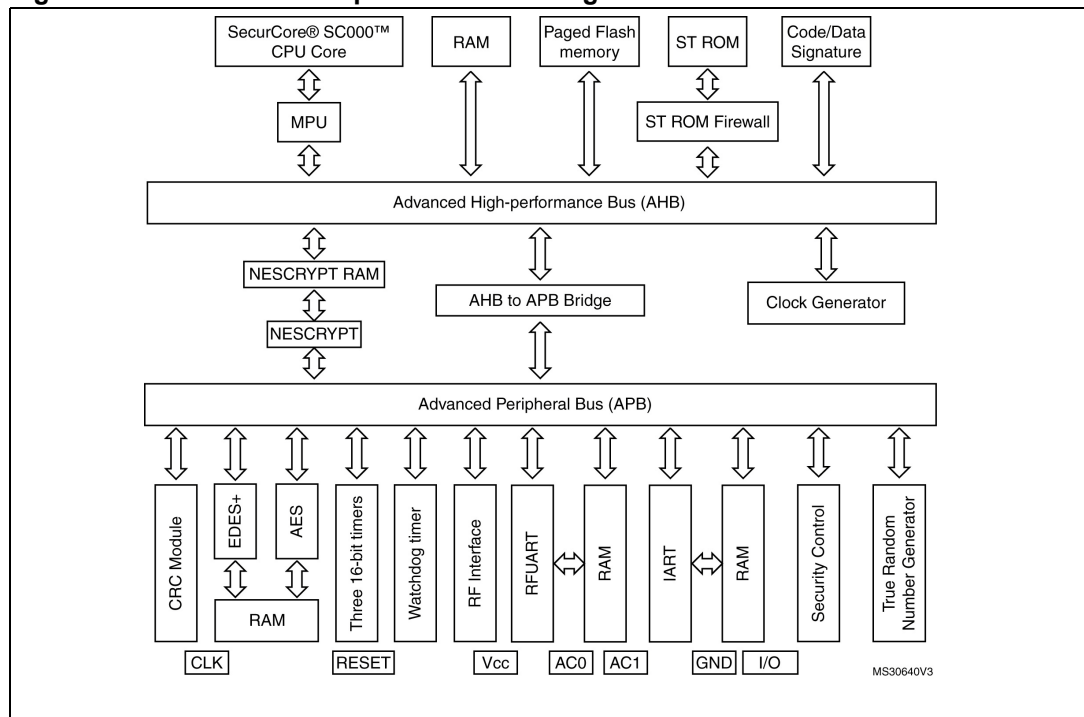
Figure 1. ST31G480 A02 platform block diagram
