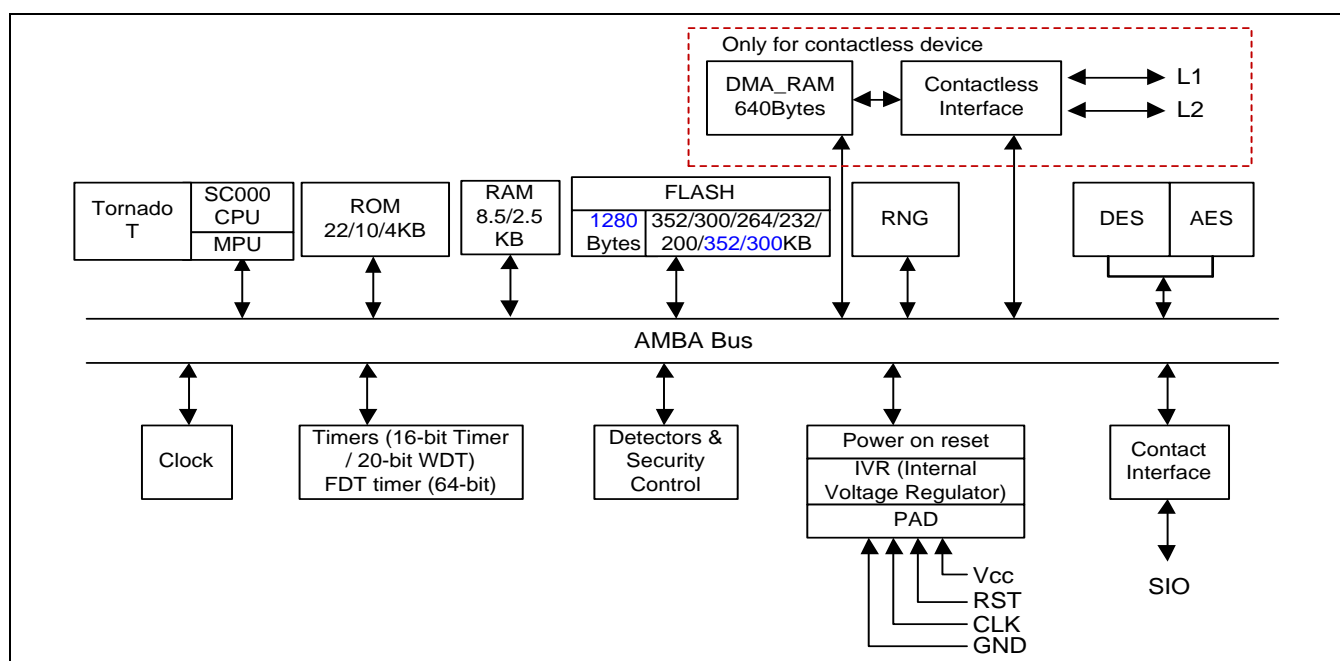
Figure 1 S3D350A/S3D300A/S3D264A/S3D232A/S3D200A/S3K350A/S3K300A Block Diagram
