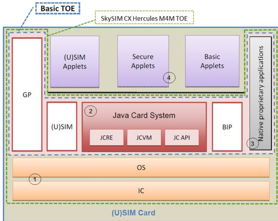
Figure 1 (U)SIM PP Basic TOE and the SkySIM CX Hercules M4M V1.0 TOE
