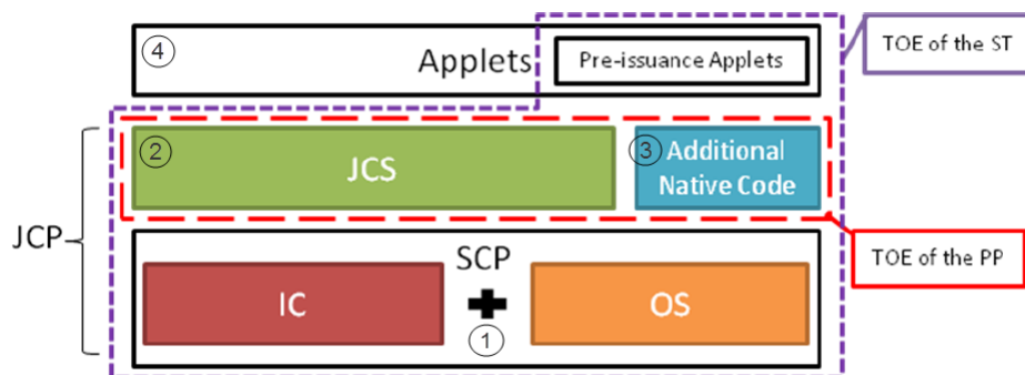
Figure 2 Java Card Platform TOE boundaries defined in JCS PP
