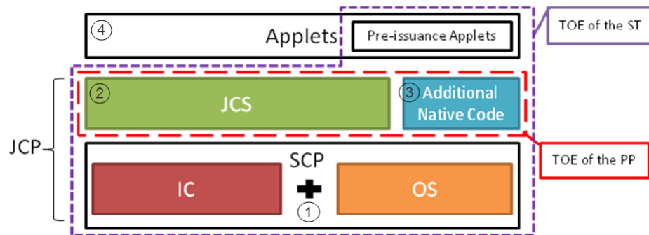
Figure 1 Sm@rtSIM CX Virgo V5.0 TOE boundaries as defined in [PPJCSv3.0], Figure 1
