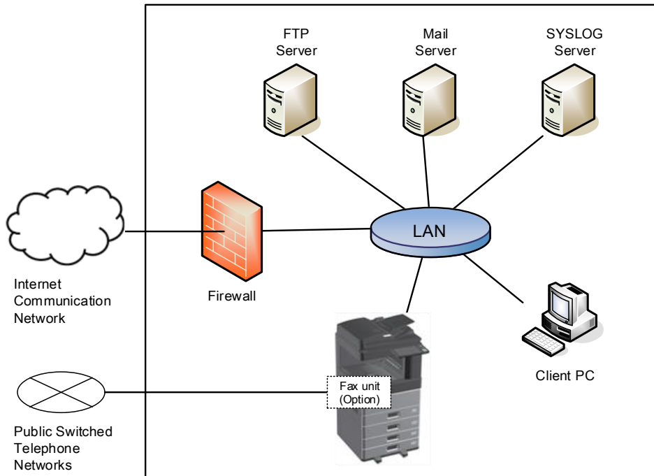
Figure 1 Environment for the usage of the MFP
