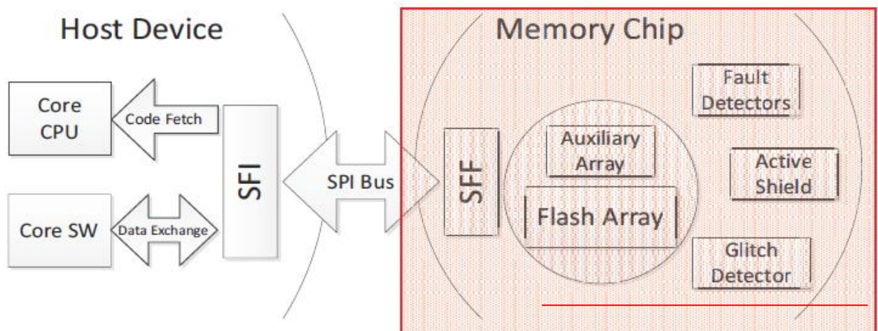
Figure 1 TOE Architecture
