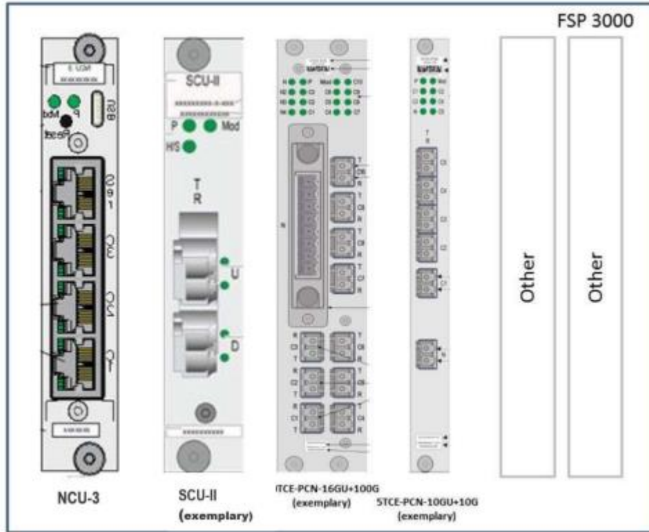
Figure 2: NCU-3 card
