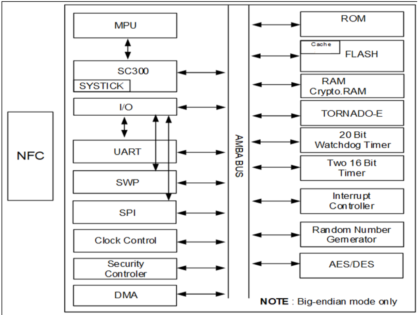
Figure 1 S3NSN4V Block Diagram
