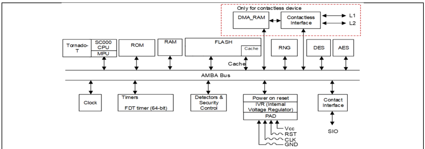
Figure 1 S3D384C/S3D352C/S3D300C/S3D264C/S3D232C/S3K384C Block Diagram
