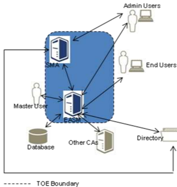
Figure 2: TOE Boundary
